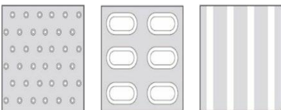
Platform edge warning paving (off-street) offset blister
